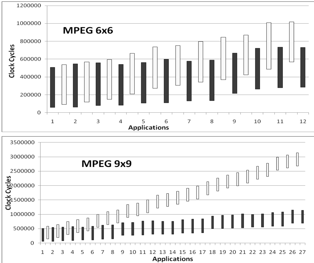
Figure 29 – Execution time for distributed (black bars) and centralized mapping (white bars), for the MPEG benchmark with two NoC sizes, scenarios B and E.
