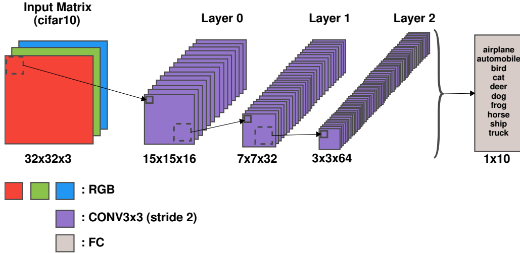
Figure 6.5: Cifar10 CNN.
