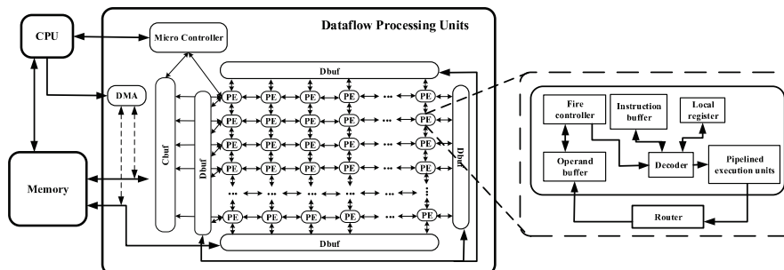
Figure 2.20: FDPU general architecture [Xiang et al., 2018].
