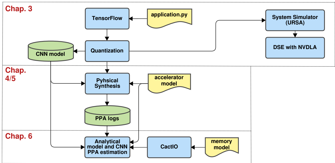
Figure 1.2: Thesis Structure.
