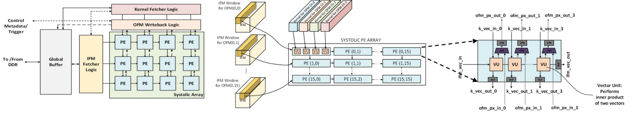
Figure 2.17: ShiDianNao accelerator architecture [Das et al., 2020].
