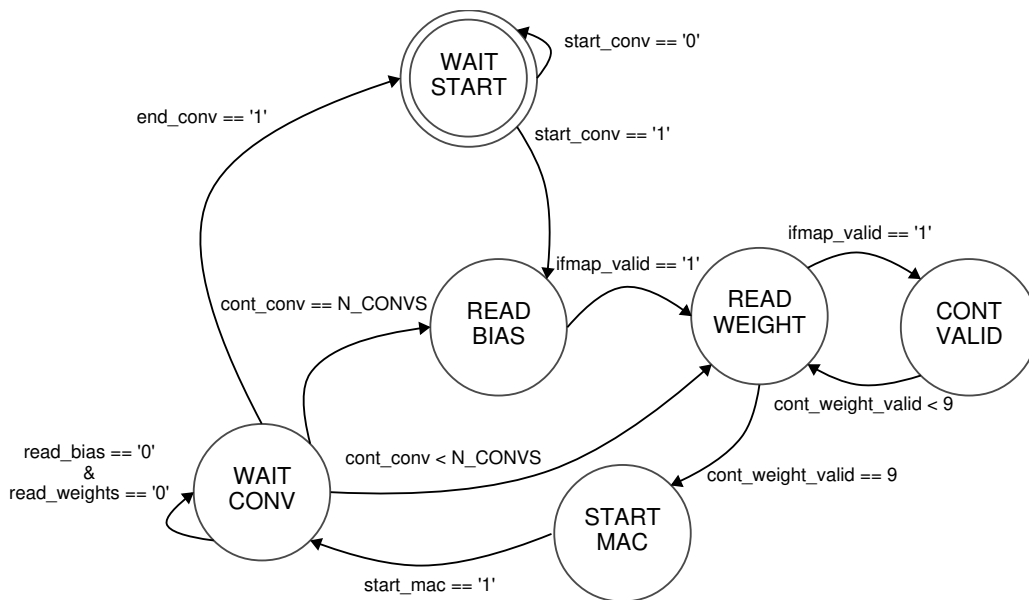
Figure 4.6: WS accelerator Control FSM.
