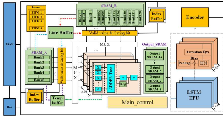
Figure 2.5: Sparsity-aware accelerator architecture [Hsiao et al., 2020].
