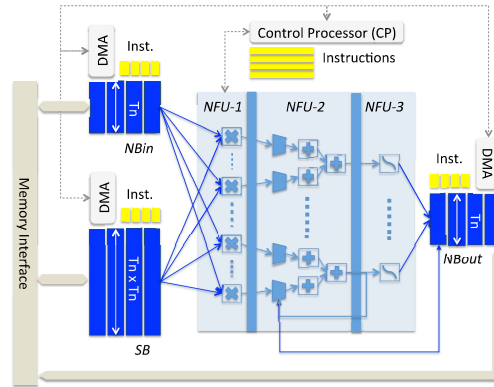
Figure 2.6: DianNao accelerator architecture [Chen et al., 2014].
